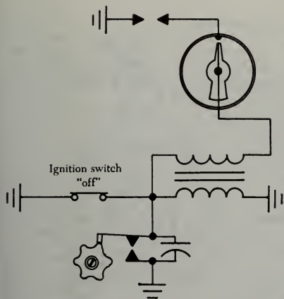
FIGURE 4-12. Typical ignition switch in "off" position.
